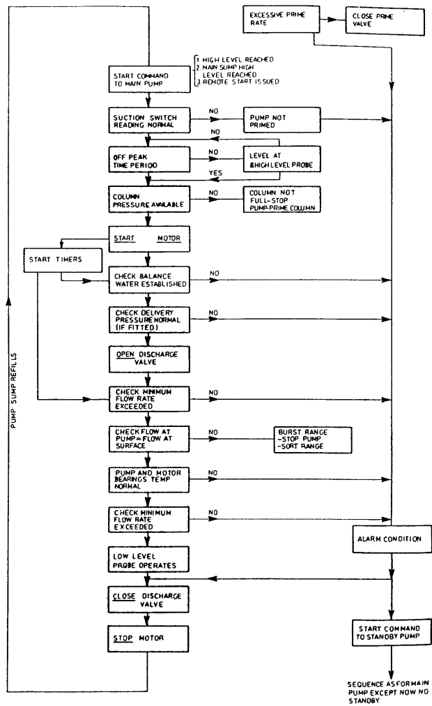
Figure 3 Start up sequence
